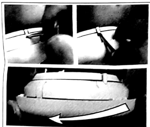
Figure 6 – Push Back the snap lock and turn the Alarm anti-clockwise
