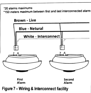
Figure 7 – Wiring & Interconnect facility
