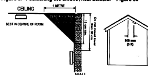
Figure 3i - Positioning the smoke / heat detector Figure 3ii
